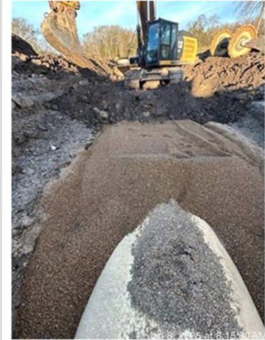
Pipe Backfill
