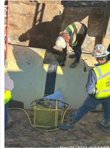
Canusa/RayChem Joint Wrapper
